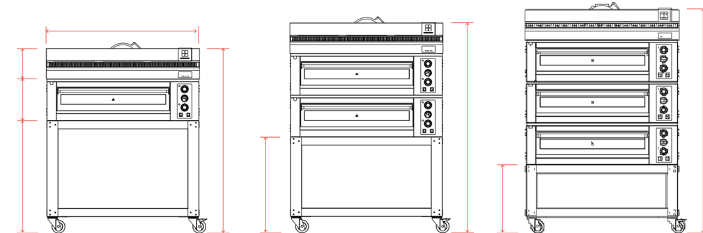
Front view / Pyralys HP 6L
