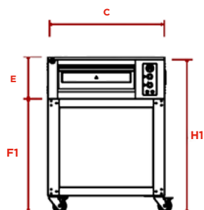
Front view / Pyralis HP 4
