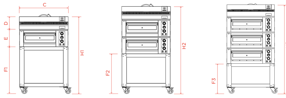
Front view / Pyralys HP 6L
