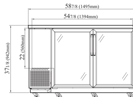
XBB-2SG-N6 FRONT VIEW
