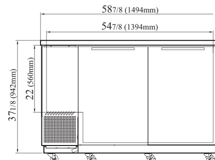
XBB-2SB-N6 FRONT VIEW
