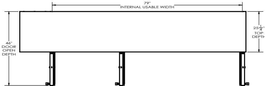
ELEVATION VIEW
