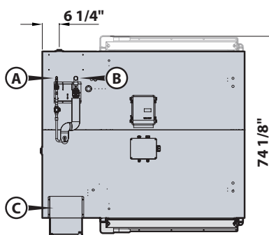
DRAIN POSITION
