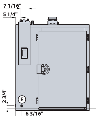
DRAIN POSITION
