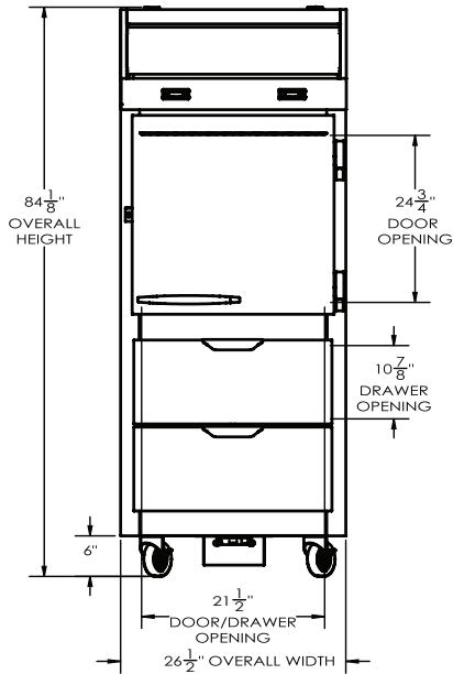
ELEVATION VIEW
