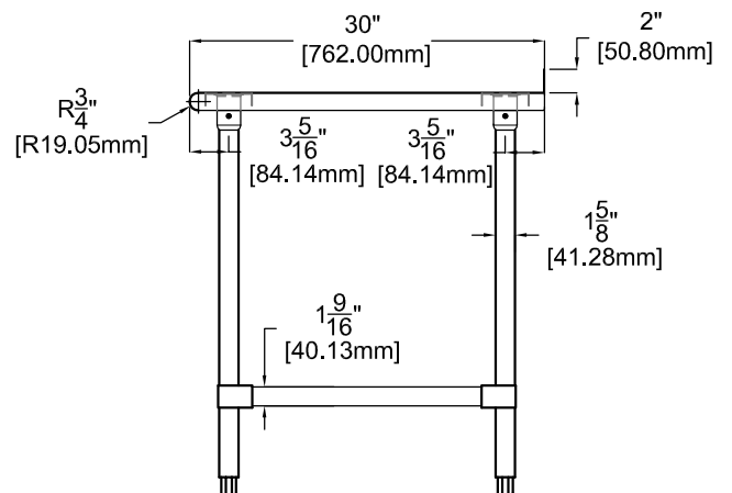
Side
