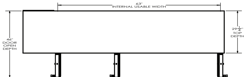
ELEVATION VIEW
