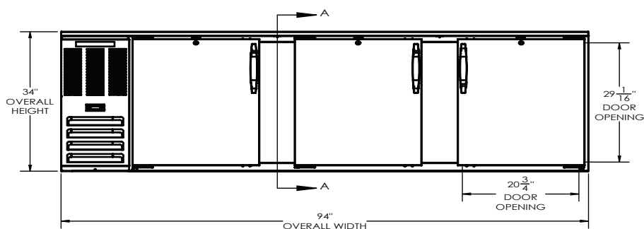
ELEVATION VIEW
