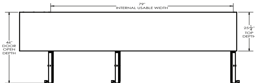
ELEVATION VIEW
