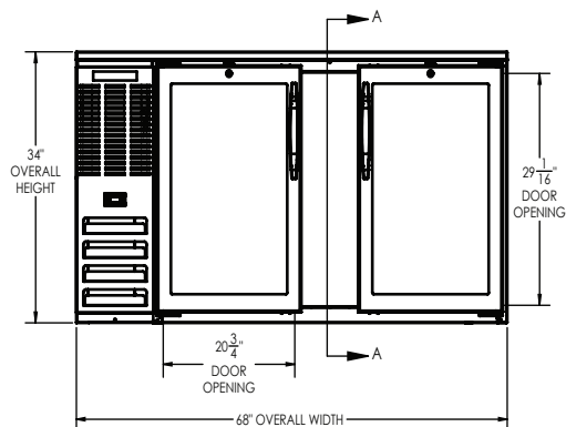
ELEVATION VIEW
