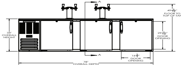
ELEVATION VIEW
