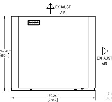
ELEVATION / FRONT VIEW
