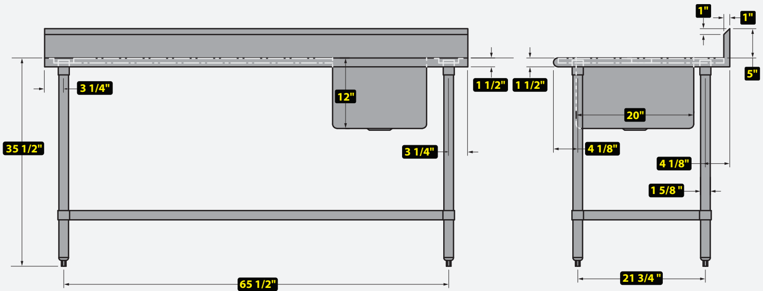
Front View
