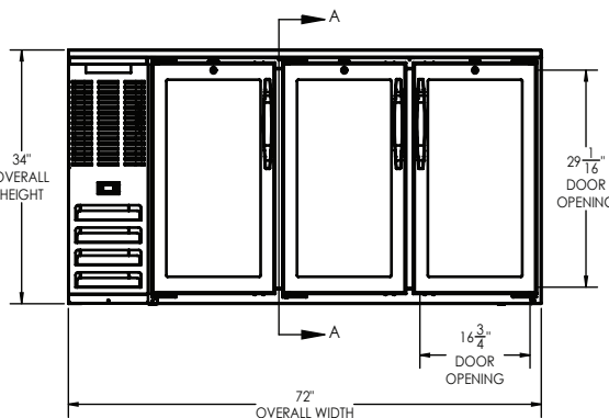
ELEVATION VIEW
