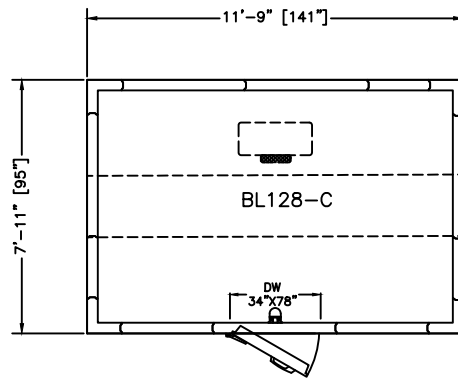
PLAN VIEW LEFT HINGE SELECT
