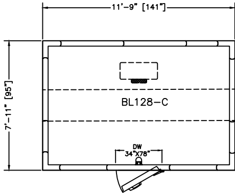
PLAN VIEW RIGHT HINGE SELECT
