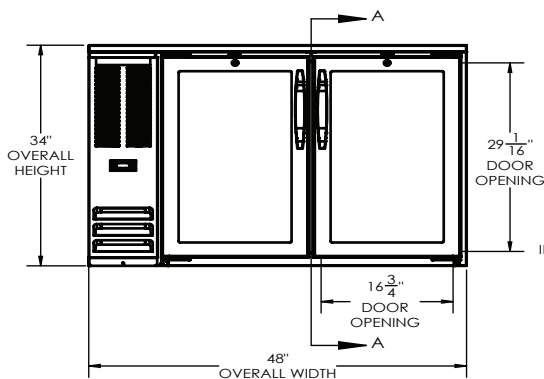
ELEVATION VIEW
