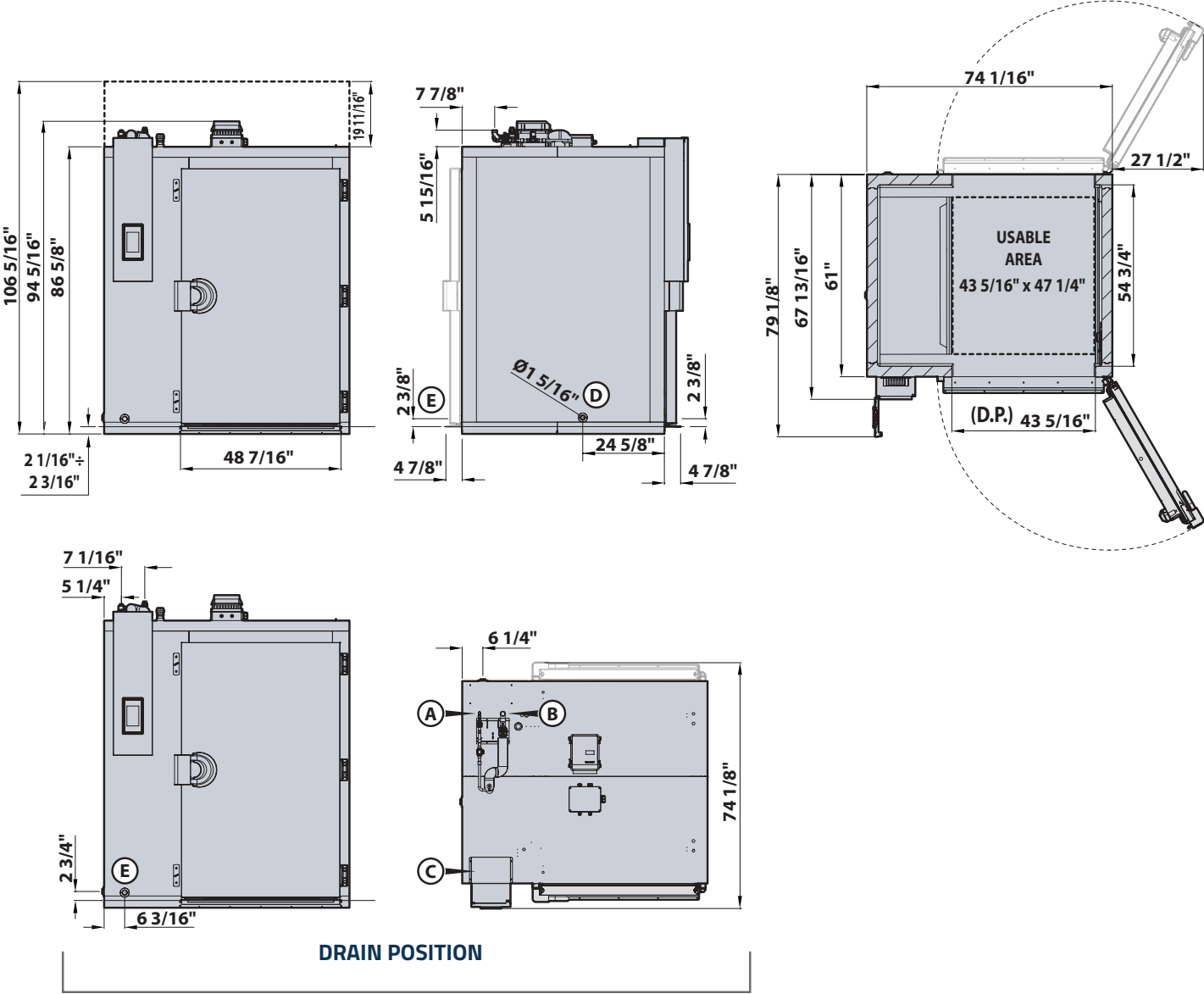
FRONT VIEW
