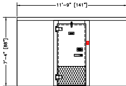
ELEVATION LEFT HINGE
