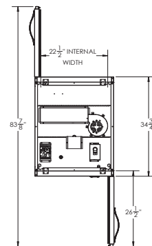
PLAN VIEW
