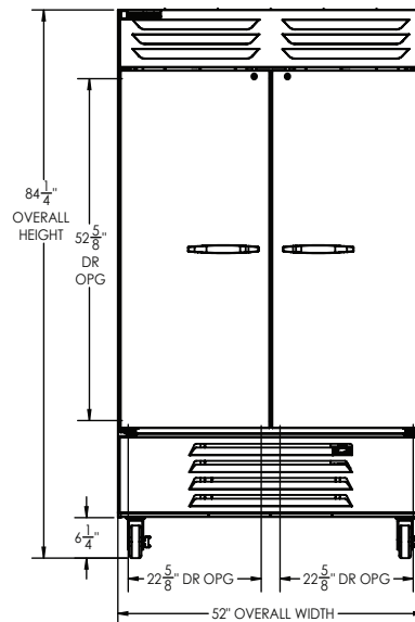
ELEVATION VIEW
