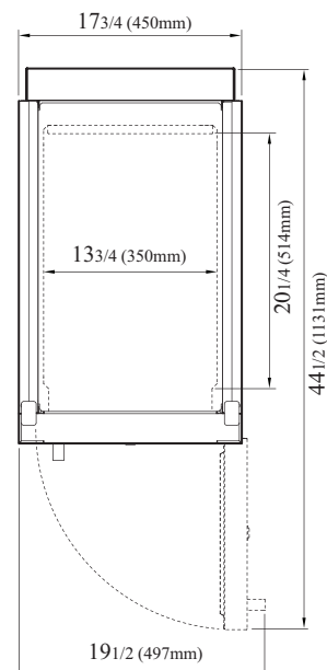
TOP VIEW
