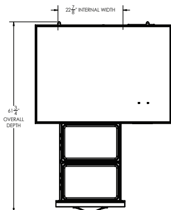
PLAN VIEW
