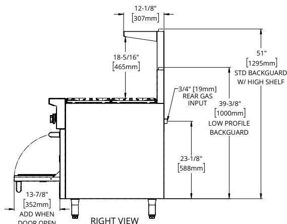
RIGHT VIEW
