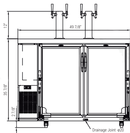
Keg configuration
