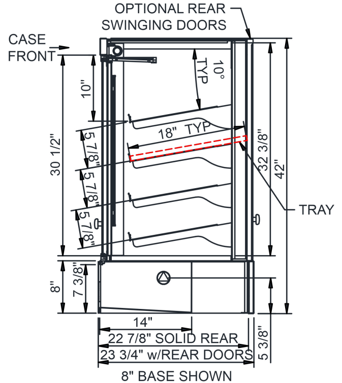
SIDE VIEW
