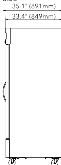
SIDE
