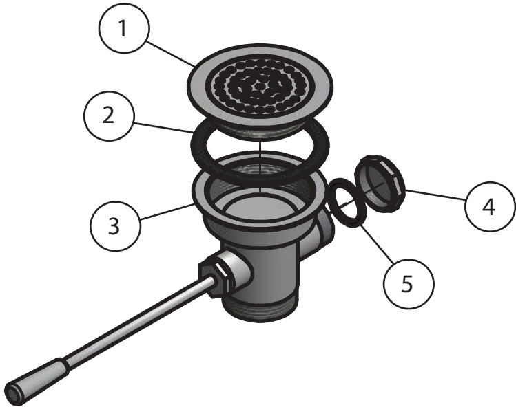
BK-SLW-2 - ISO VIEW Scale = 1:6
