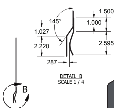
BK-FSS - SIDE VIEW Scale = 1:10
