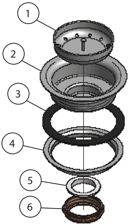
BKDR-4 - ISO VIEW Scale = 1:3
