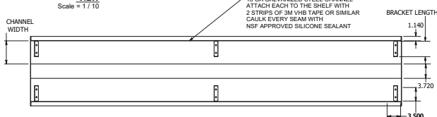
BOTTOM VIEW Scale = 1 / 10
