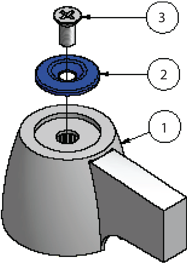
BKF-DBH - ISO VIEW
