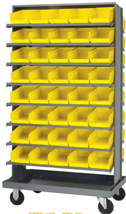
QPRD-102 + QDU-00 Mobile, Double Sided Pick Rack Up to 1,200 lb. mobile load capacity. 2 rigid, 2 swivel with brake hard rubber casters.
