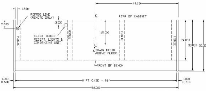
8 FOOT CASE 98"
