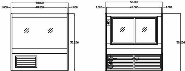
SC-CDS,CMS,CFS32-4
