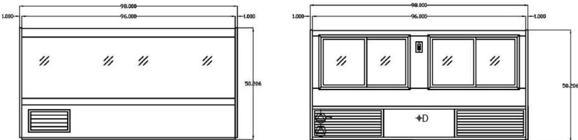
SC-CDS,CMS,CFS32-8
