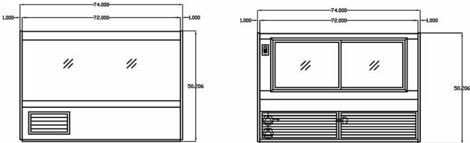
SC-CDS,CMS,CFS32-6
