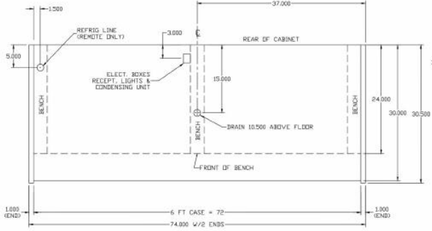
6 FOOT CASE 74"
