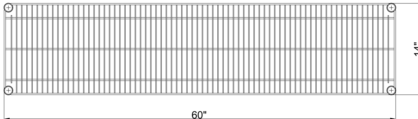
Top View
