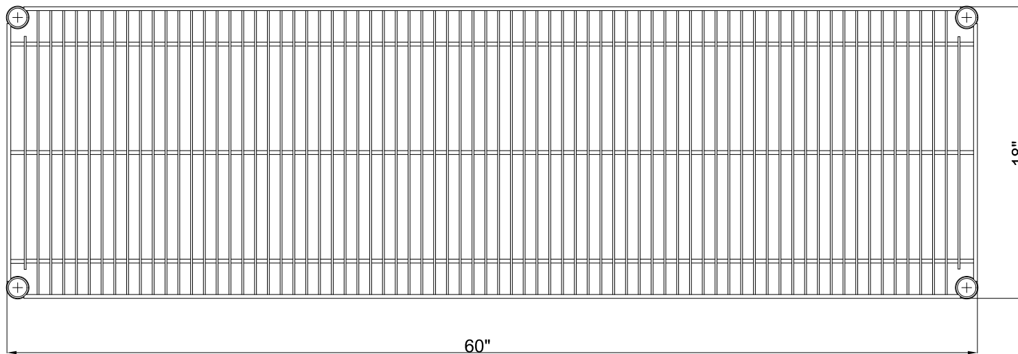
Top View
