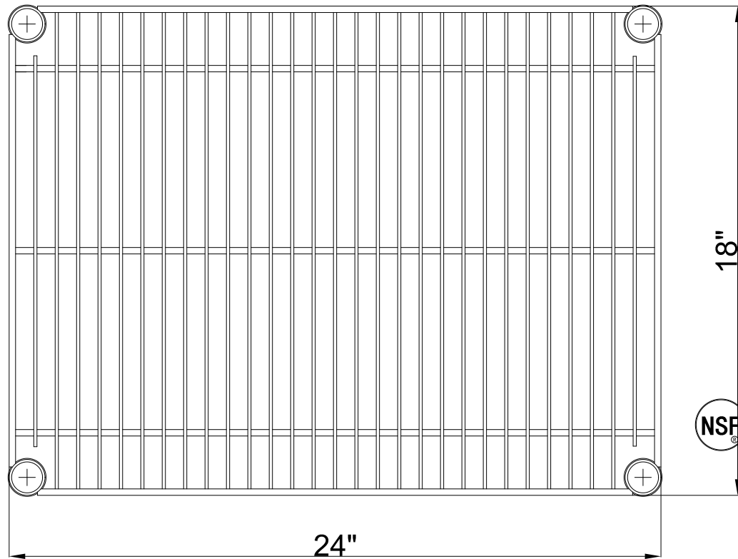
Top View
