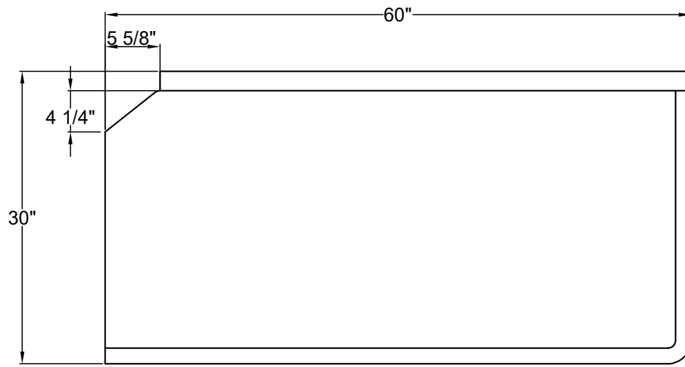
Top View
