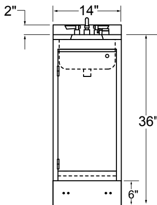
PLAN VIEW
