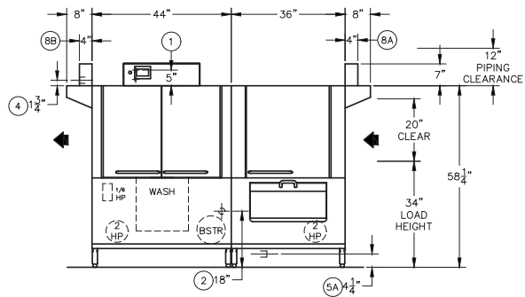
Front View: Right to Left Model
