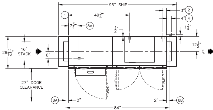
Plan View: Left to Right Model
