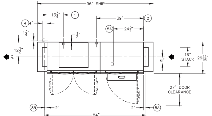
Plan View: Right to Left Model
