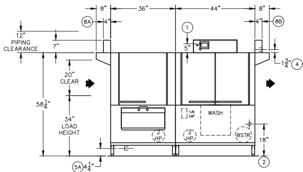
Front View: Left to Right Model
