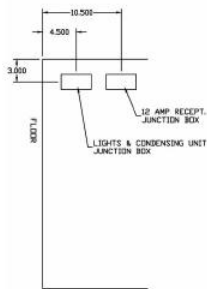
JUNCTION BOX
