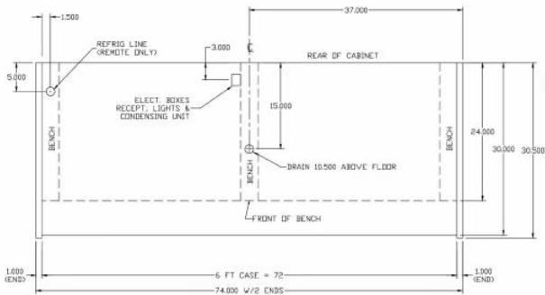
6 FOOT CASE 74"
