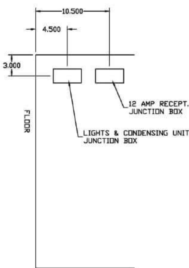
JUNCTION BOX
