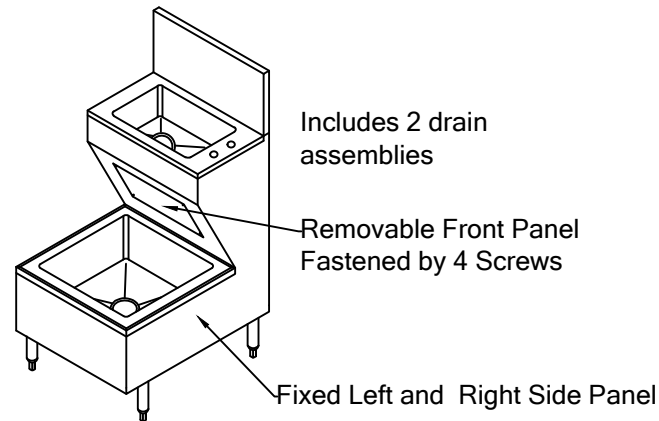
ISOMETRIC
