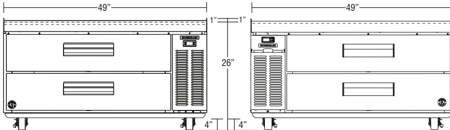
CR49B shown
