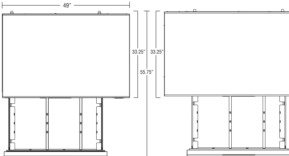
CR49B shown
