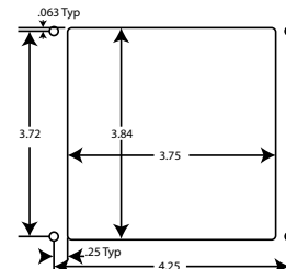
Control Cutout
