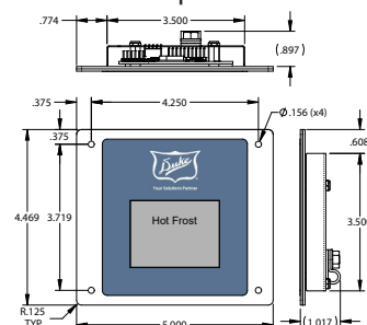
Control Cutout
