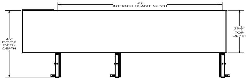
ELEVATION VIEW
