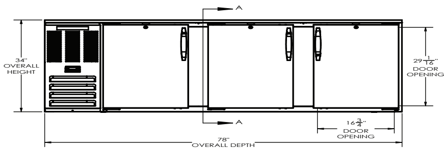
ELEVATION VIEW
