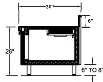
SECTION VIEW
