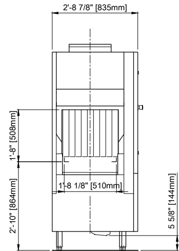
Side Elevation View
