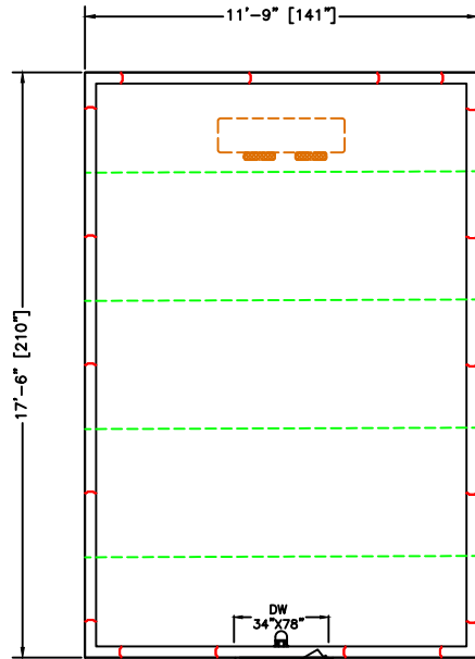
PLAN VIEW RIGHT HINGE SELECT
