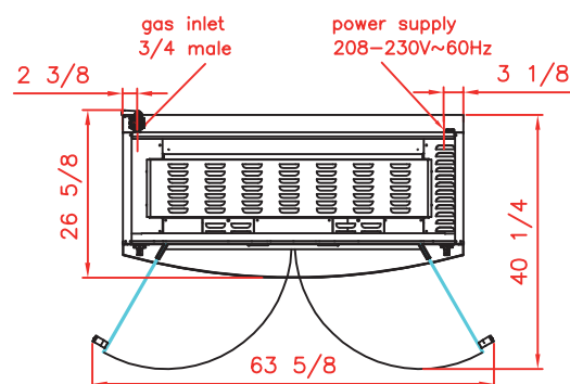
Top view Rotisserie with roof
