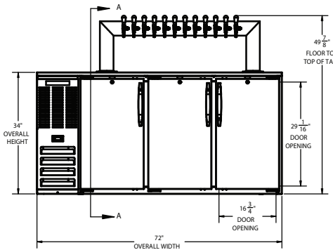
ELEVATION VIEW
