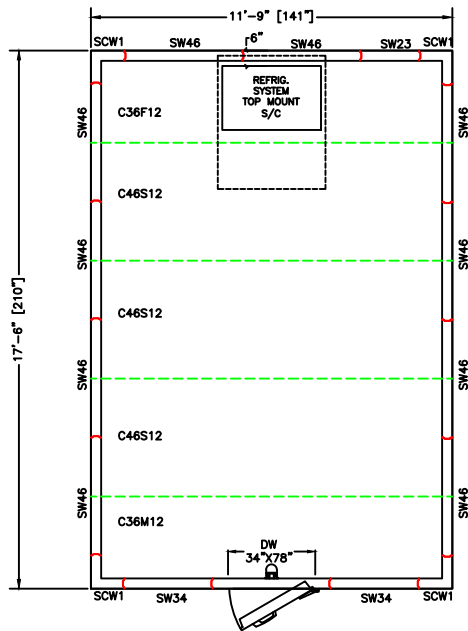
PLAW VIEW RIGHT HINGE SELECT
