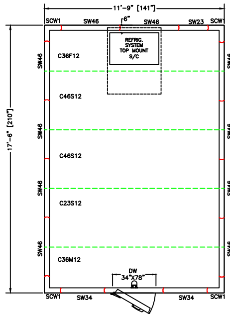
PLAW VIEW LEFT HINGE SELECT
